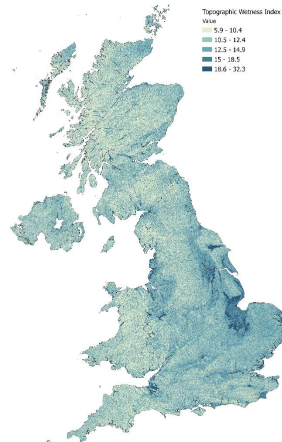
Figure 5. TWI calculated for mainland UK. Note: areas of accumulation in upland peat-rich soils are under-represented by TWI (see Section 4).
